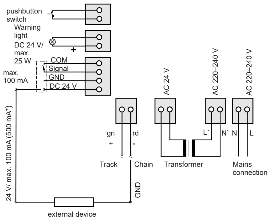
Fig. Connection diagram ceiling control unit
