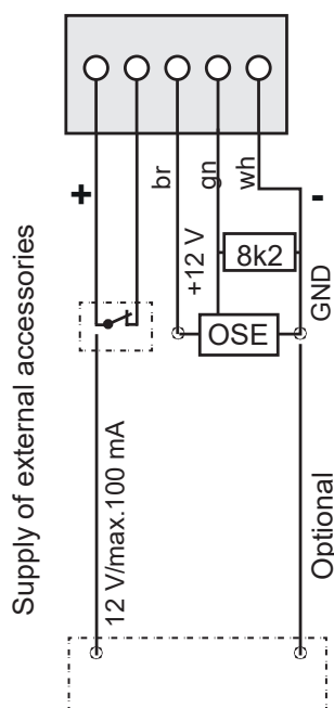
Fig. Connection diagram, motor carriage
